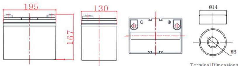
Terminal Dimensions
